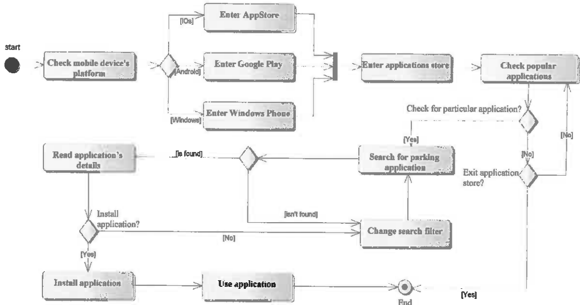
Fig. 1. Standard installation scenario of mobile application
