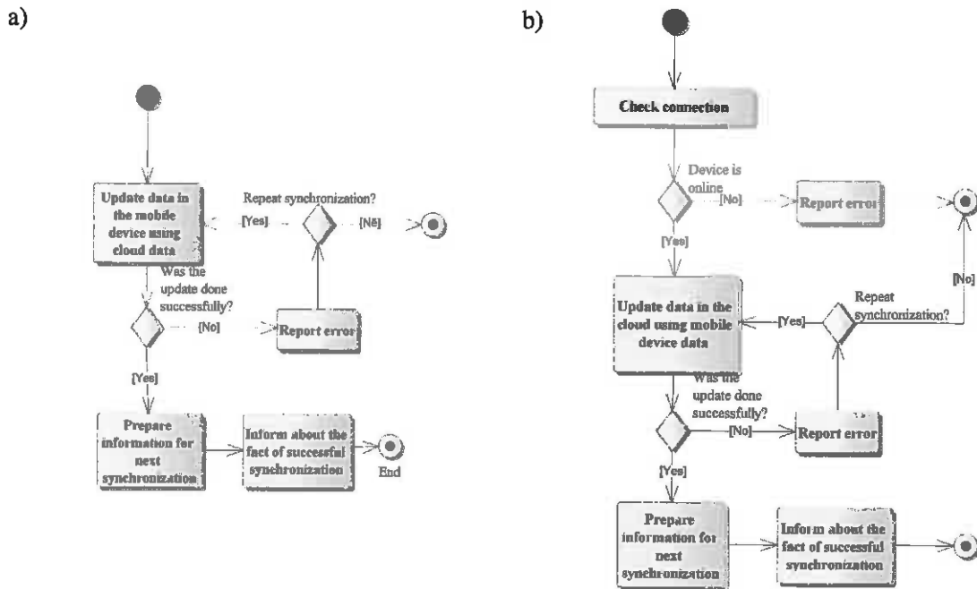
Fig. 2. Slow synchronization scenario: a – mobile device-cloud synchronization; b – cloud-mobile device synchronization
