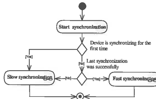
Fig. 4. Decision of synchronization scenario
