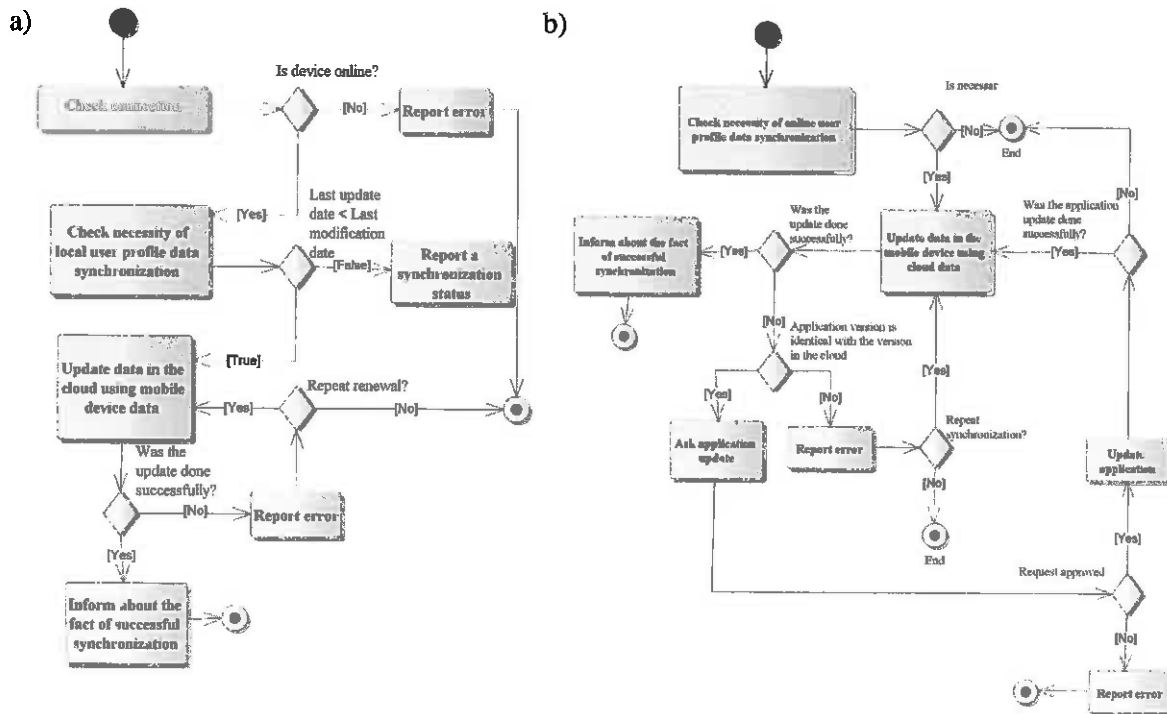
Fig. 3. Fast synchronization scenario: a – mobile device-cloud synchronization; 2 – cloud-mobile device synchronization
